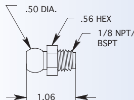
1/8" MALE CONNECTOR
