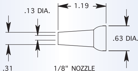
1/8" NOZZLE
