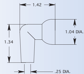
1/4" 90 DEGREE NOZZLE
