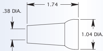
3/8" NOZZLE
