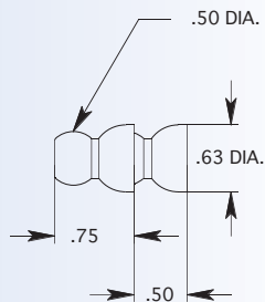
1/4" BODY SEGMENTS
