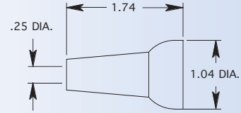
1/2" X 1/4" DRIP-RESISTANT NOZZLE
