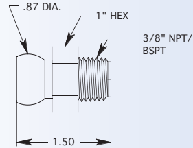
3/8" MALE CONNECTOR
