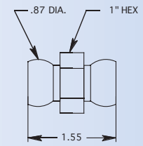
1/2" DOUBLE BALL ADAPTER
