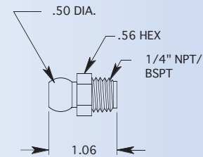
1/4" MALE CONNECTOR
