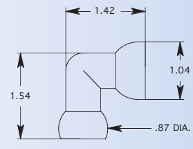
1/2" 90 DEGREE ELBOW
