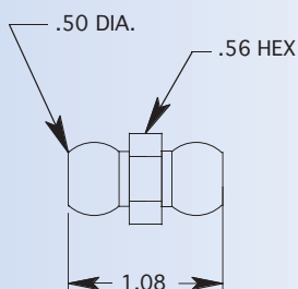
1/4" DOUBLE BALL ADAPTER
