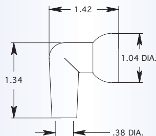
3/8" 90 DEGREE NOZZLE
