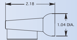
1/2" SIDE-SPRAY NOZZLE
