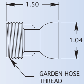
MALE GARDEN HOSE X FEMALE SNAP-LOC ADPTR
