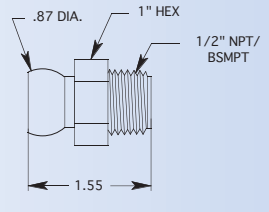
1/2" MALE CONNECTOR
