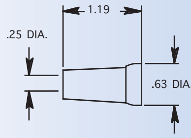
1/4" NOZZLE
