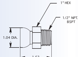
1/2" F HOSE X 1/2" CONNECTOR
