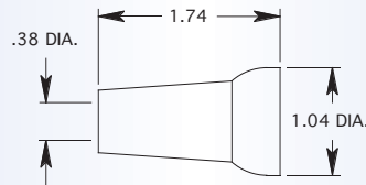
1/2" X 3/8" DRIP-RESISTANT NOZZLE
