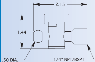
1/4" HOSE X 1/4" F NPT/F BSPT VALVE
