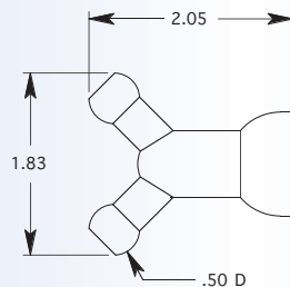
1/2" X 1/4" REDUCER Y - MOLDED STYLE
