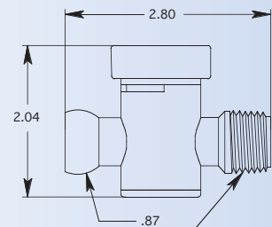
1/2" MALE NPT/BSPT X FEMALE NPT/BSPT VALVE
