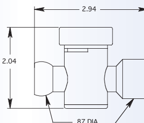
1/2" HOSE X FEMALE NPT/BSPT VALVE
