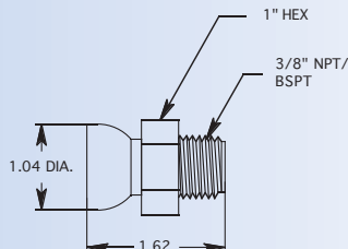
1/2" F HOSE X 3/8" CONNECTOR
