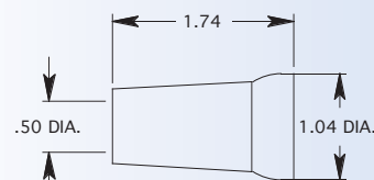
1/2" NOZZLE
