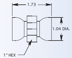
1/2" DOUBLE SOCKET ADAPTER
