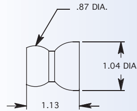
1/2" IN-LINE CHECK VALVE
