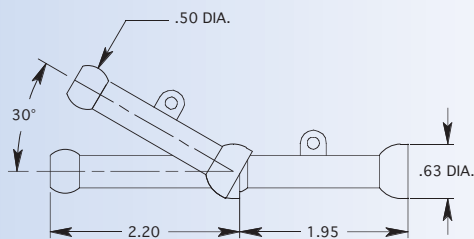
1/4" EXTENSION SEGMENTS
