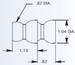
1/2" BODY SEGMENTS
