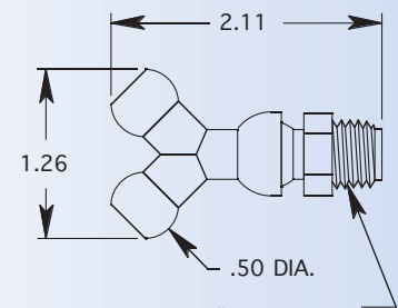
1/4" Y X 1/8" & 1/4" CONNECTOR MOLDED
