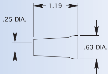
1/4" X 1/4" DRIP-RESISTANT NOZZLE
