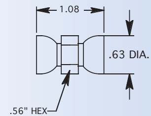
1/4" DOUBLE SOCKET ADAPTER
