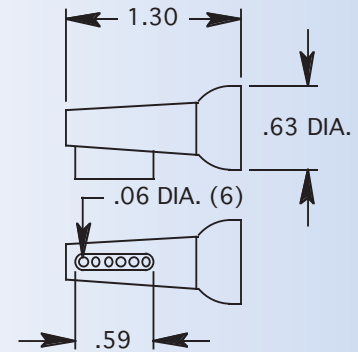
1/4" SIDE-SPRAY NOZZLE
