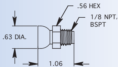
1/4" F HOSE X 1/8" CONNECTOR
