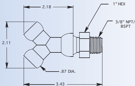
1/2" Y X 3/8" CONNECTOR
