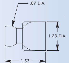
FEMALE GARDEN HOSE X MALE SNAP-LOC ADPTR
