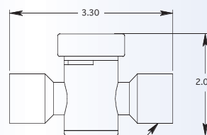
1/2" F NPT/F BSPT (2) 1/2" FEMALE NPT/BSPT X FEMALE NPT/F BSPT VALVE
