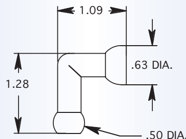
1/4" 90 DEGREE ELBOW
