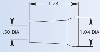
1/2" X 1/2" DRIP-RESISTANT NOZZLE
