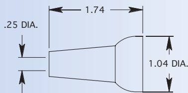
1/4" NOZZLE
