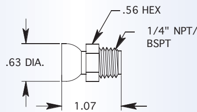
1/4" F HOSE X 1/4" CONNECTOR
