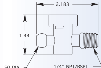
1/4" HOSE X 1/4" NPT/BSPT VALVE
