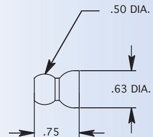
1/4" IN-LINE CHECK VALVE
